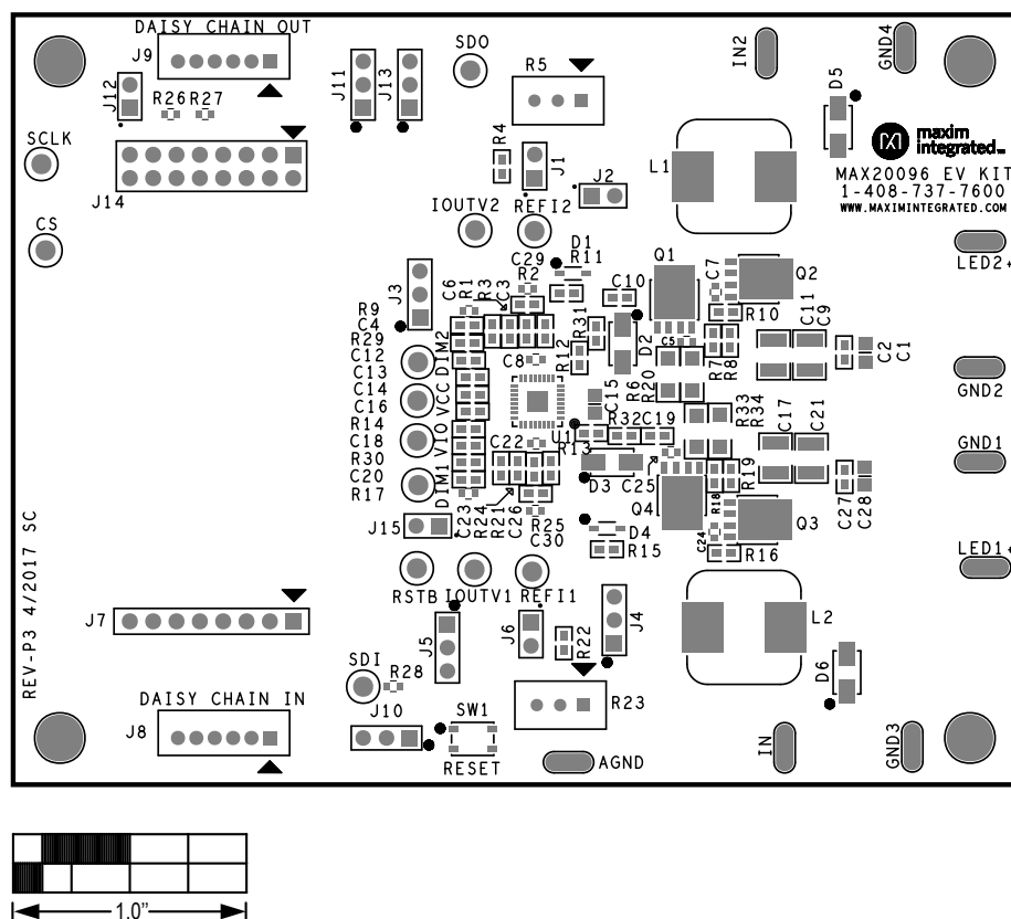
MAX20096 EV Kit Component Placement Guide—Component Side
