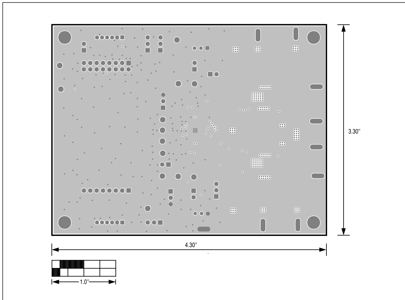
MAX20096 EV Kit PCB Layout—Inner Layer 1
